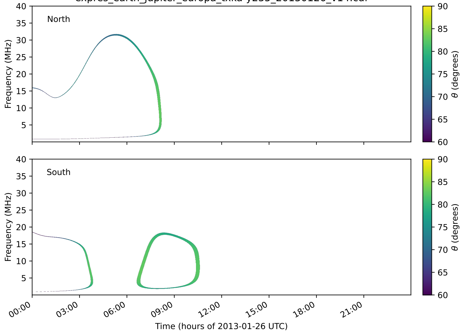
expres_earth_jupiter_europa_txka-y235_20130126_v14.cdf
