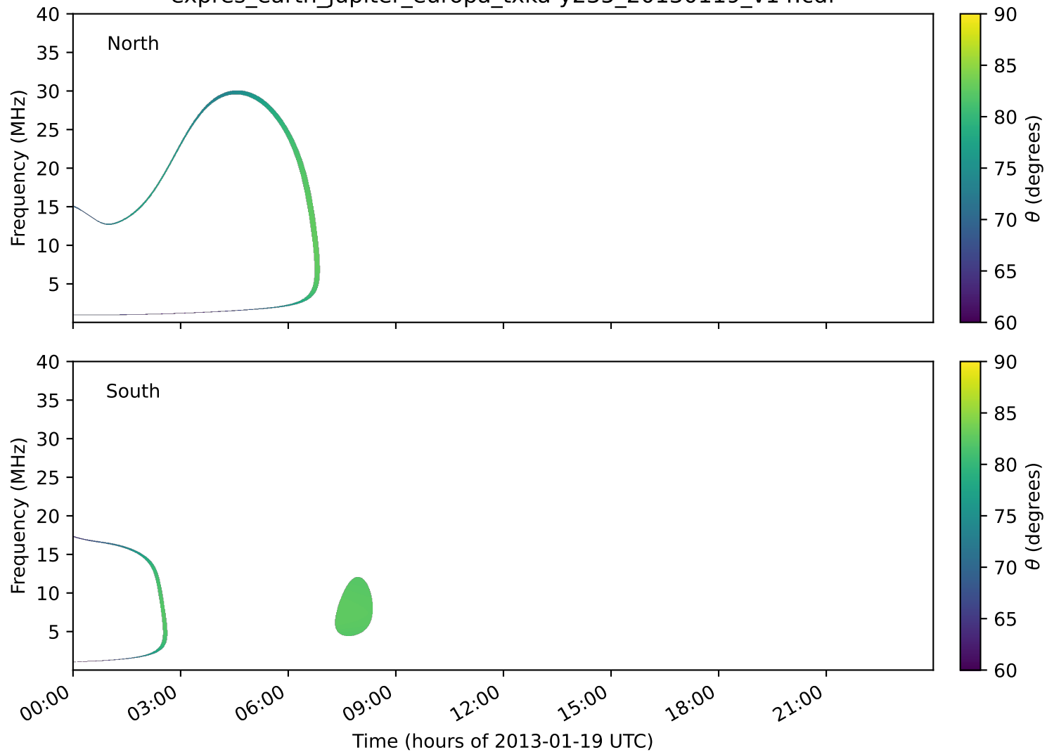
expres_earth_jupiter_europa_txka-y235_20130119_v14.cdf
