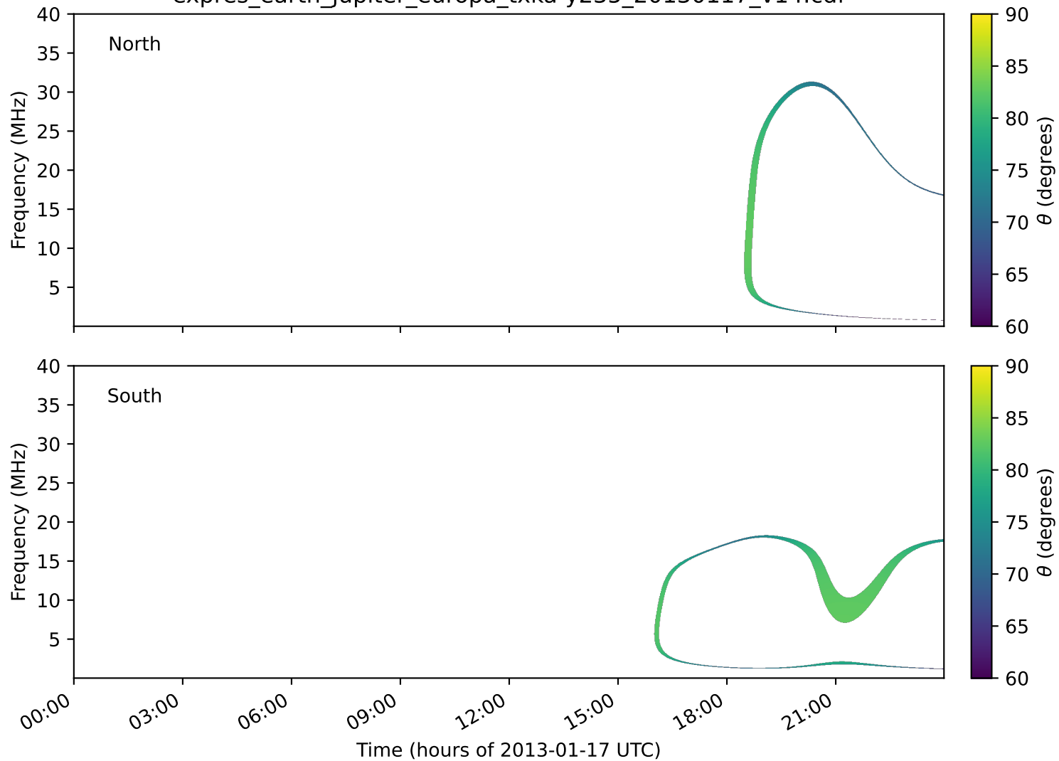
expres_earth_jupiter_europa_txka-y235_20130117_v14.cdf
