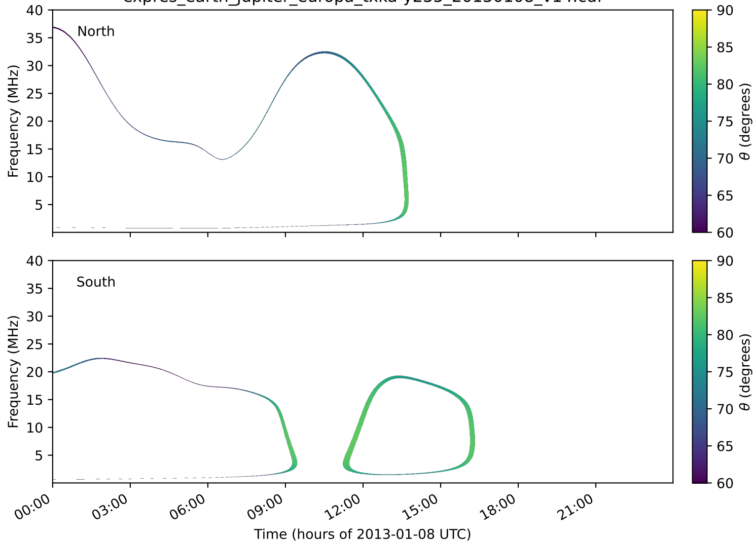
expres_earth_jupiter_europa_txka-y235_20130108_v14.cdf
