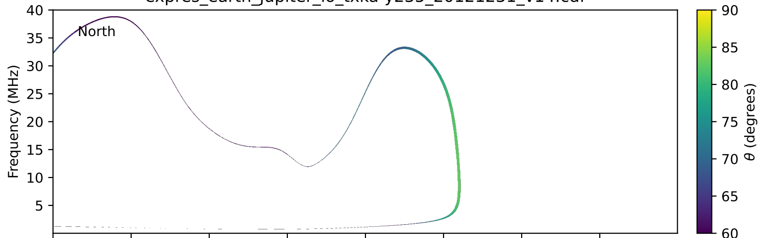
expres_earth_jupiter_io_txka-y235_20121231_v14.cdf
