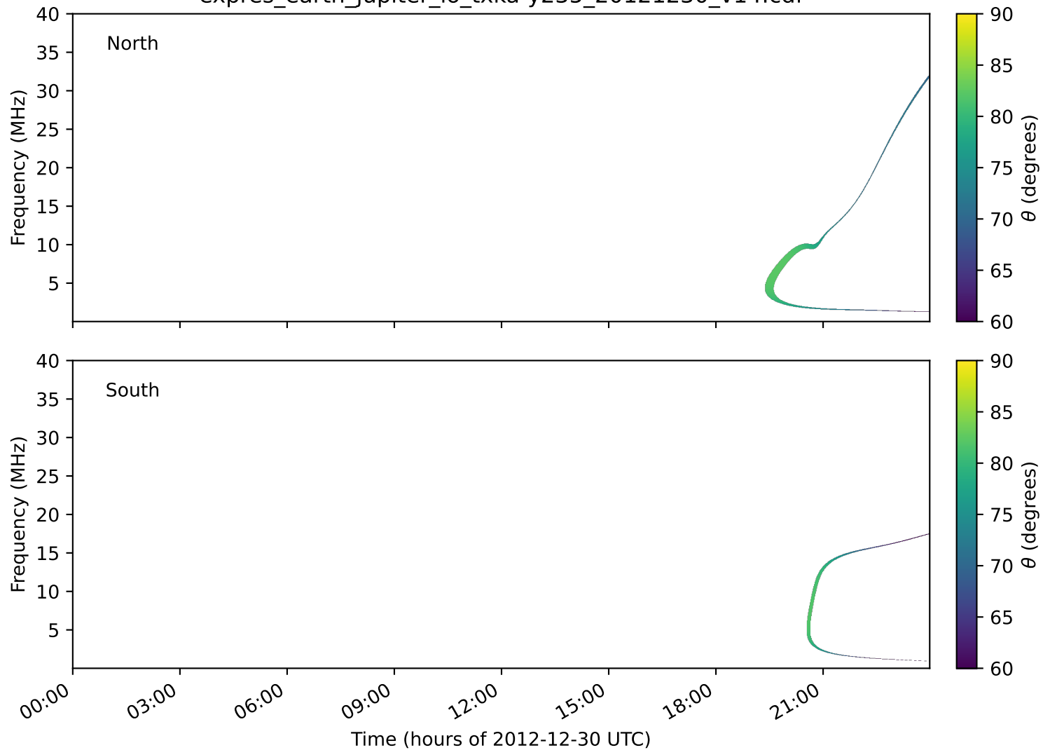
expres_earth_jupiter_io_txka-y235_20121230_v14.cdf
