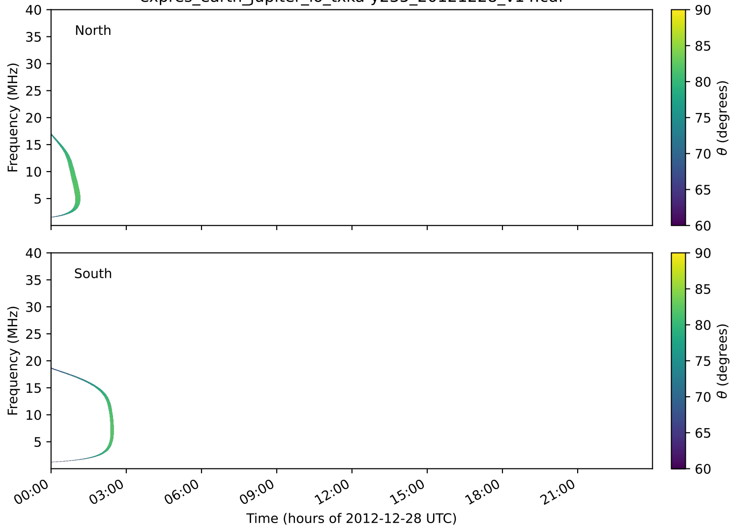
expres_earth_jupiter_io_txka-y235_20121228_v14.cdf
