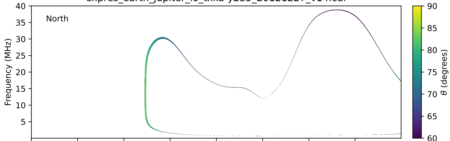
expres_earth_jupiter_io_txka-y235_20121227_v14.cdf
