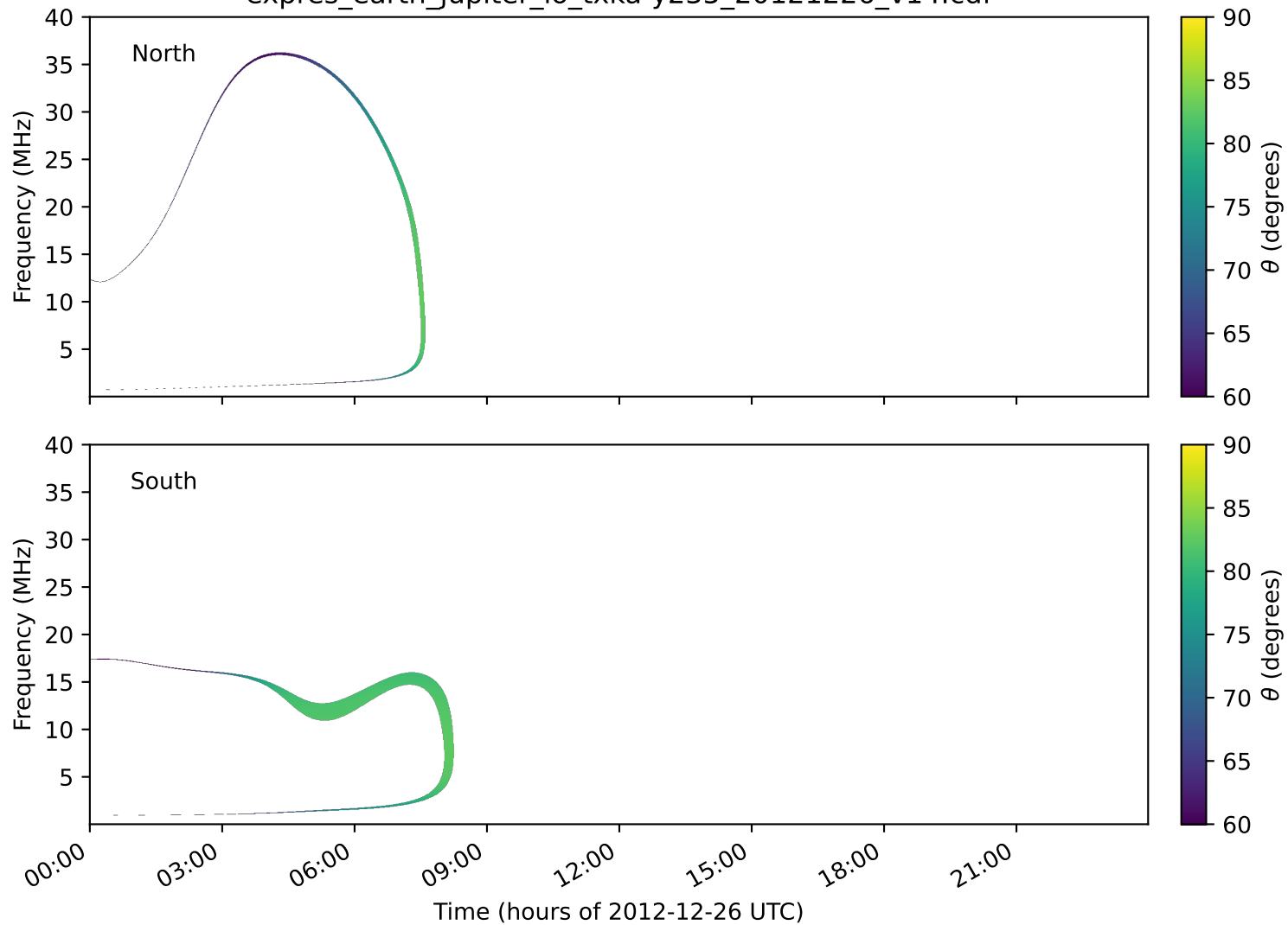
expres_earth_jupiter_io_txka-y235_20121226_v14.cdf
