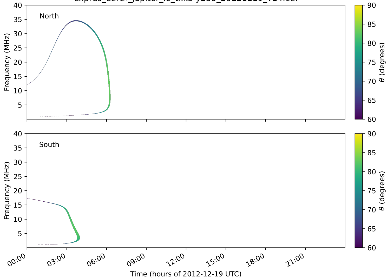
expres_earth_jupiter_io_txka-y235_20121219_v14.cdf
