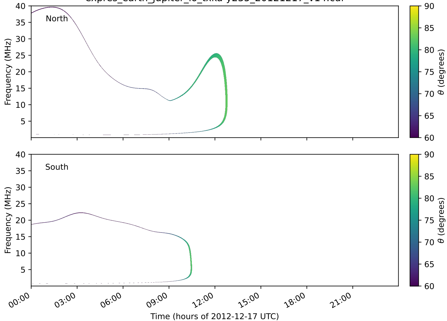
expres_earth_jupiter_io_txka-y235_20121217_v14.cdf
