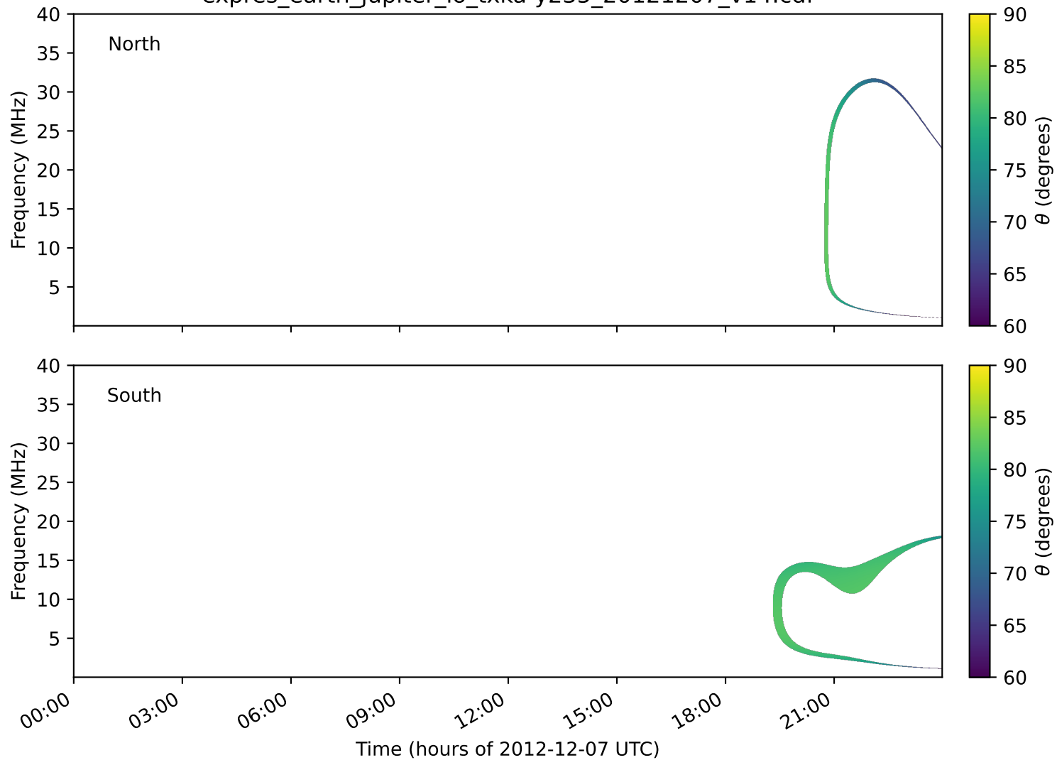
expres_earth_jupiter_io_txka-y235_20121207_v14.cdf
