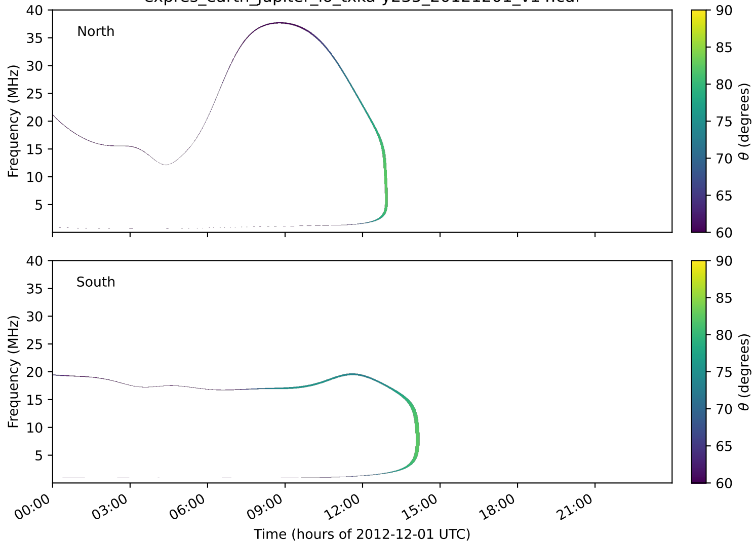
expres_earth_jupiter_io_txka-y235_20121201_v14.cdf
