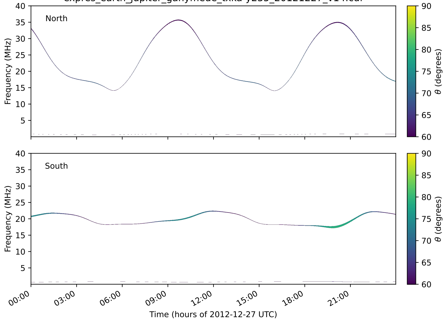
expres_earth_jupiter_ganymede_txka-y235_20121227_v14.cdf
