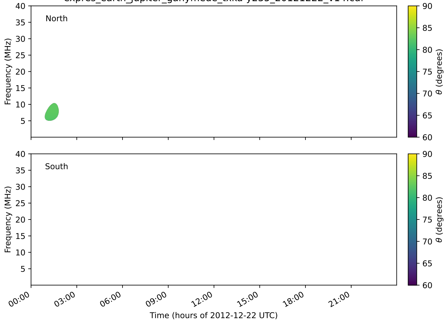
expres_earth_jupiter_ganymede_txka-y235_20121222_v14.cdf
