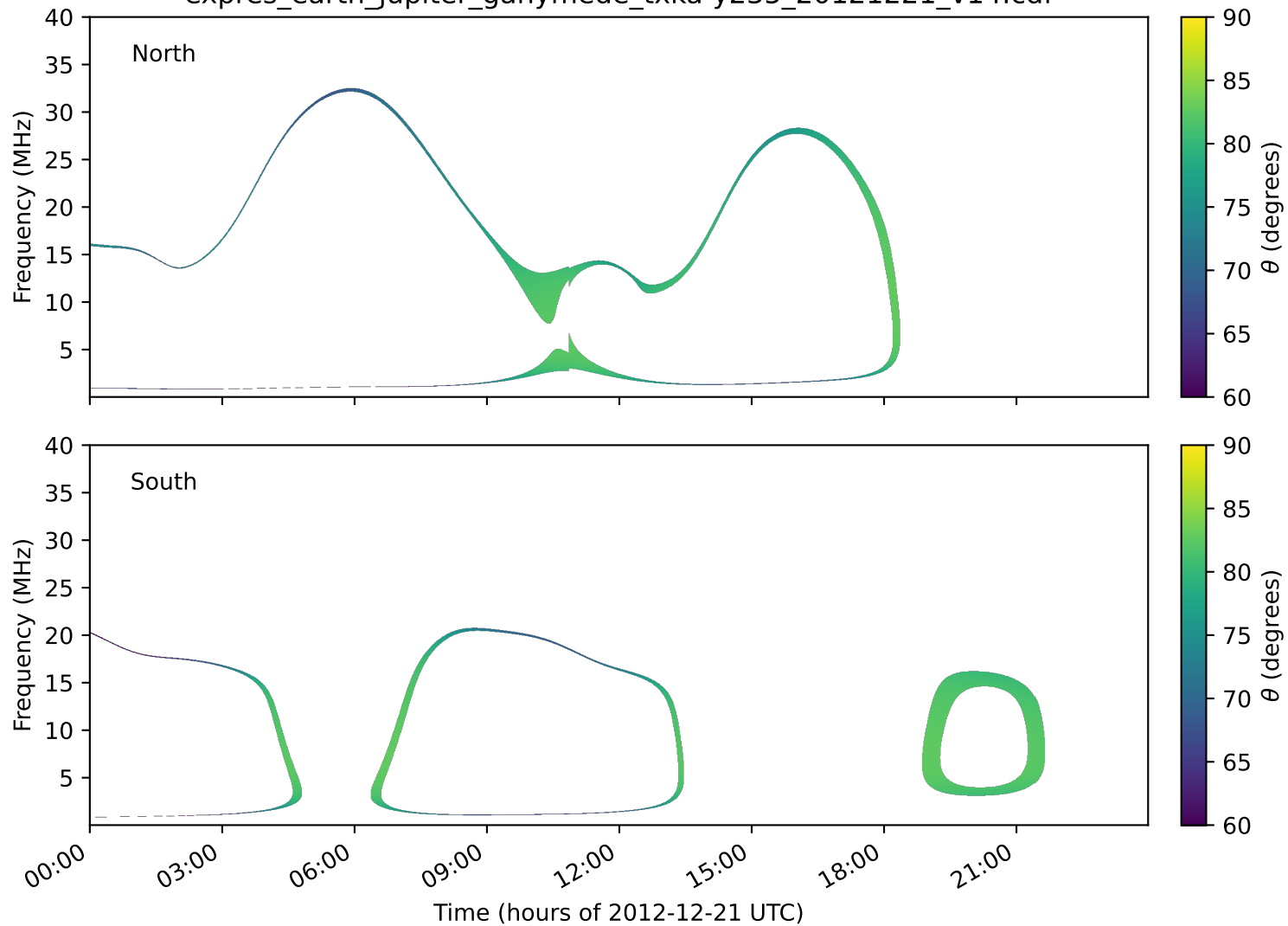
expres_earth_jupiter_ganymede_txka-y235_20121221_v14.cdf
