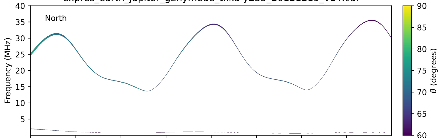
expres_earth_jupiter_ganymede_txka-y235_20121219_v14.cdf
