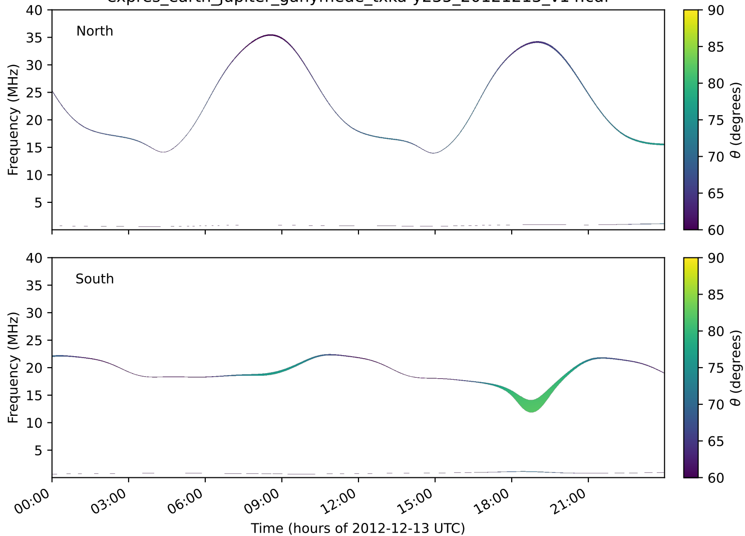
expres_earth_jupiter_ganymede_txka-y235_20121213_v14.cdf
