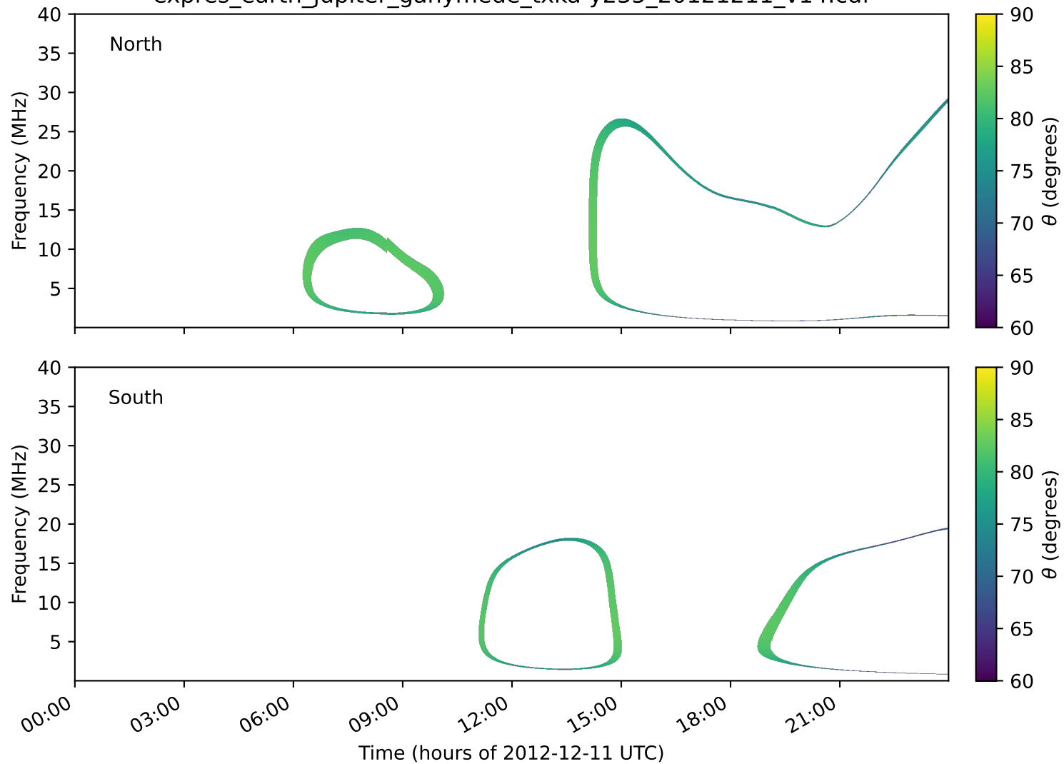
expres_earth_jupiter_ganymede_txka-y235_20121211_v14.cdf
