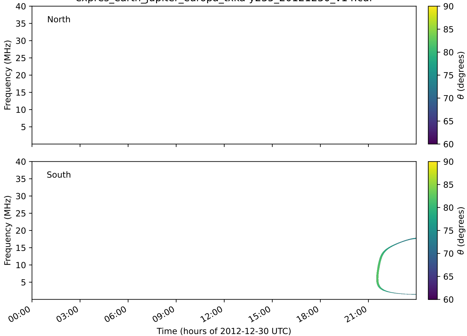
expres_earth_jupiter_europa_txka-y235_20121230_v14.cdf
