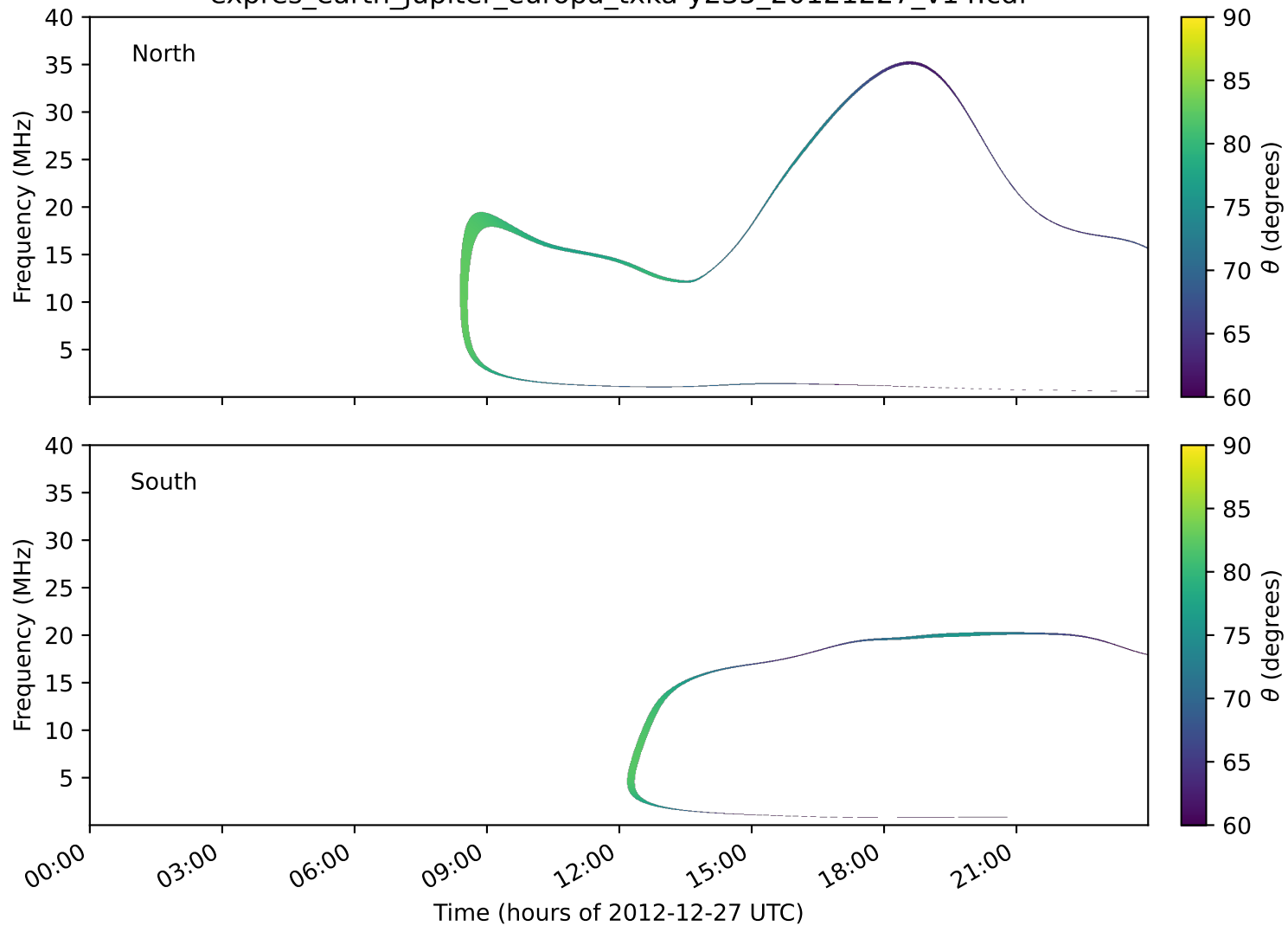
expres_earth_jupiter_europa_txka-y235_20121227_v14.cdf
