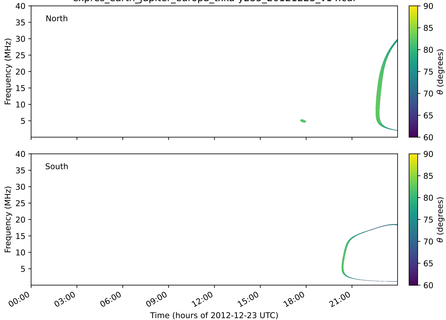
expres_earth_jupiter_europa_txka-y235_20121223_v14.cdf
