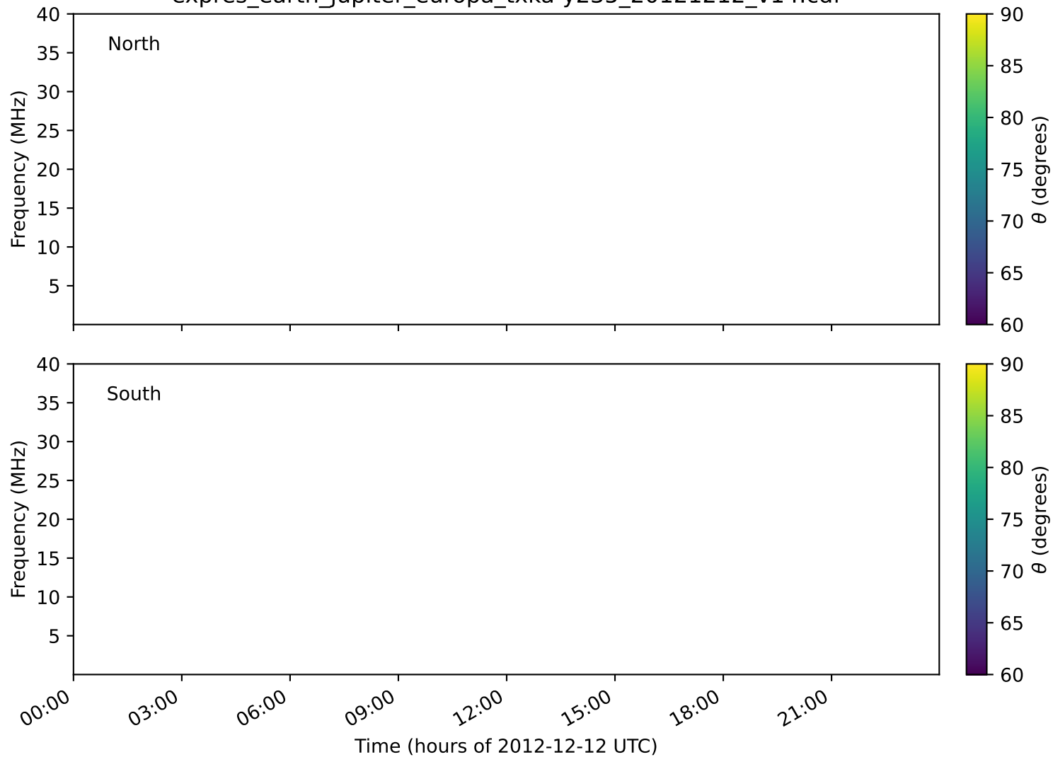
expres_earth_jupiter_europa_txka-y235_20121212_v14.cdf
