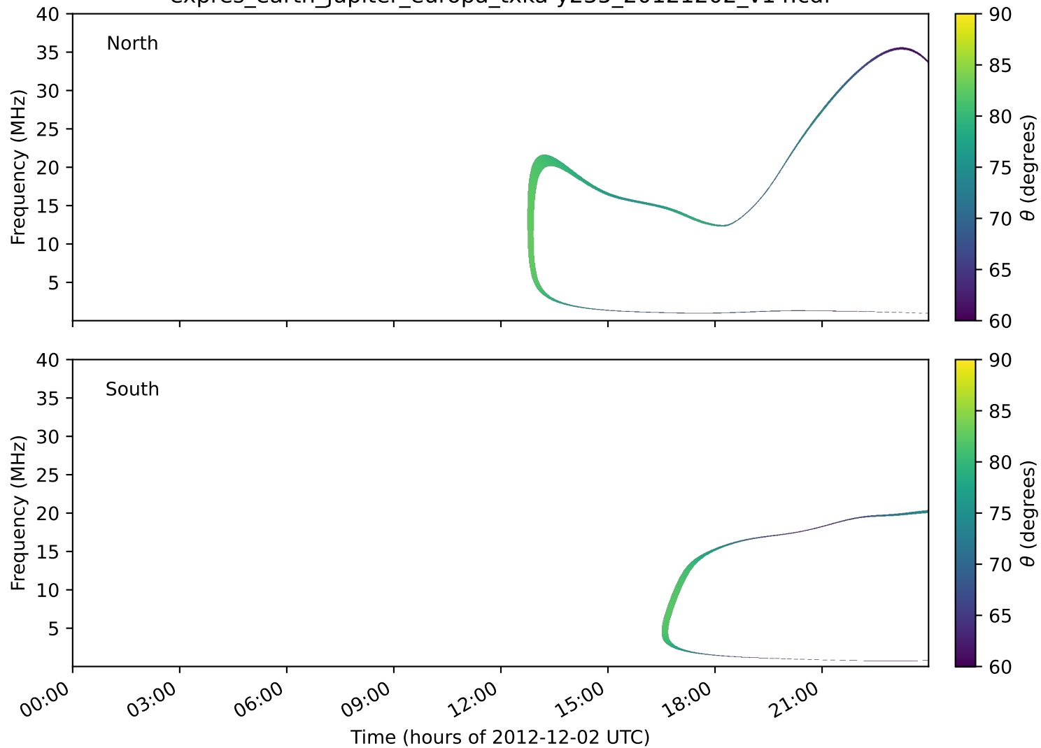
expres_earth_jupiter_europa_txka-y235_20121202_v14.cdf
