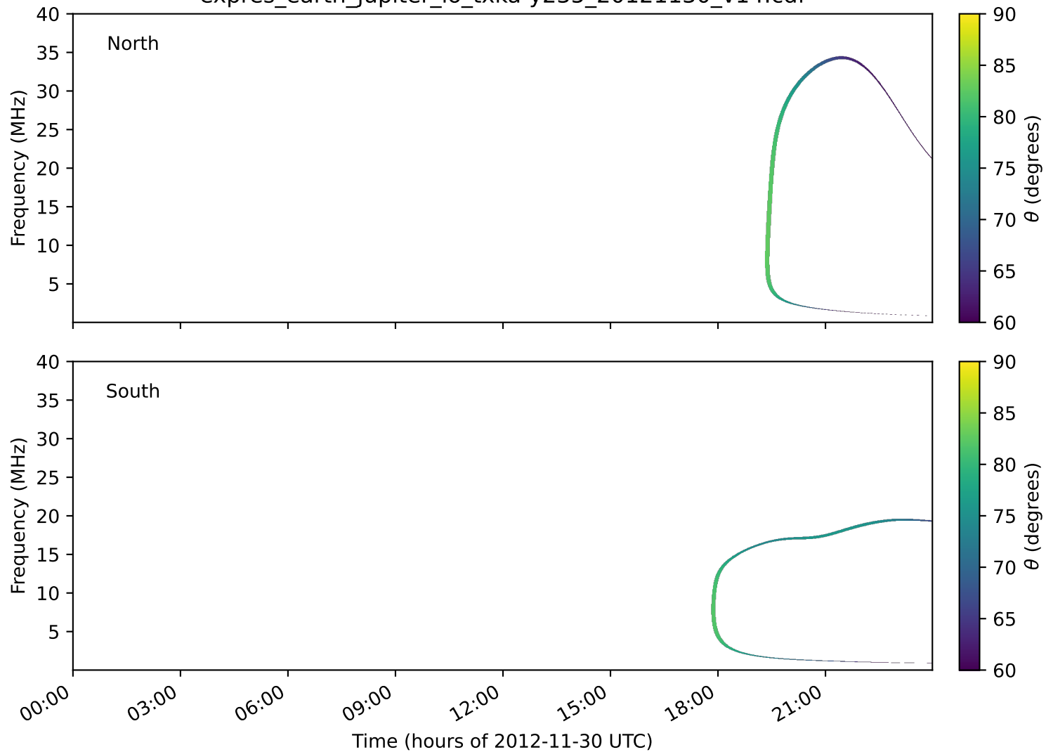
expres_earth_jupiter_io_txka-y235_20121130_v14.cdf
