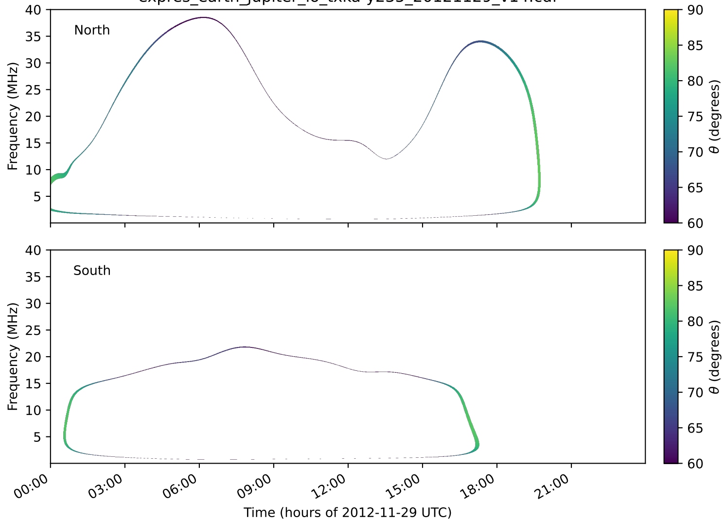
expres_earth_jupiter_io_txka-y235_20121129_v14.cdf
