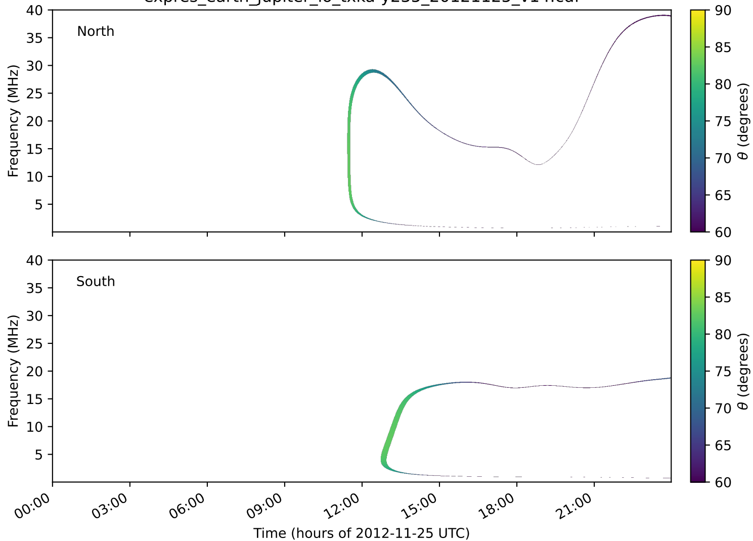
expres_earth_jupiter_io_txka-y235_20121125_v14.cdf
