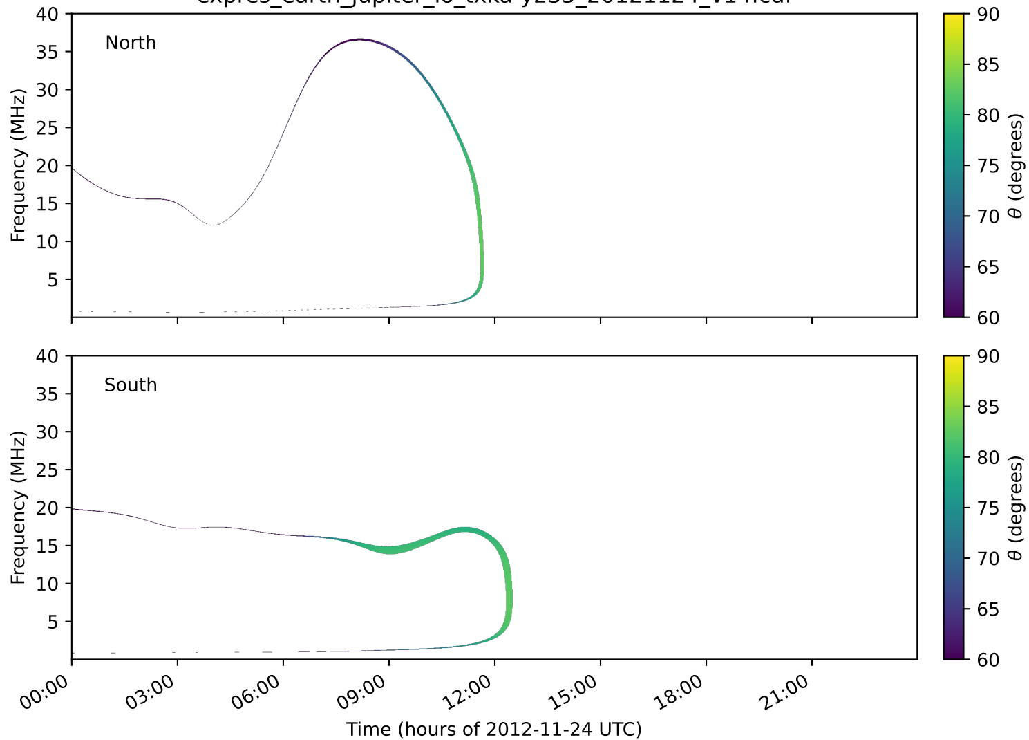
expres_earth_jupiter_io_txka-y235_20121124_v14.cdf
