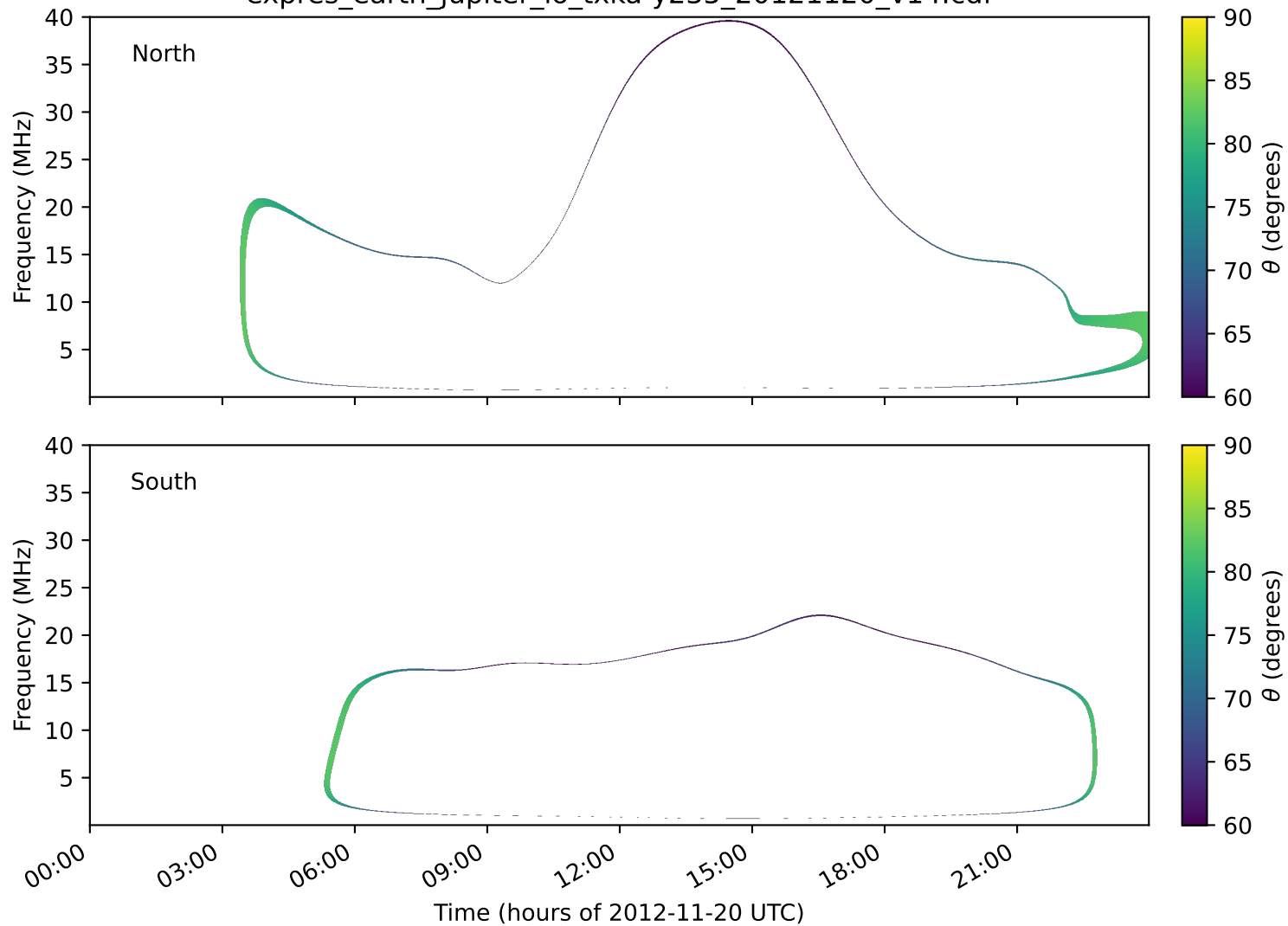
expres_earth_jupiter_io_txka-y235_20121120_v14.cdf
