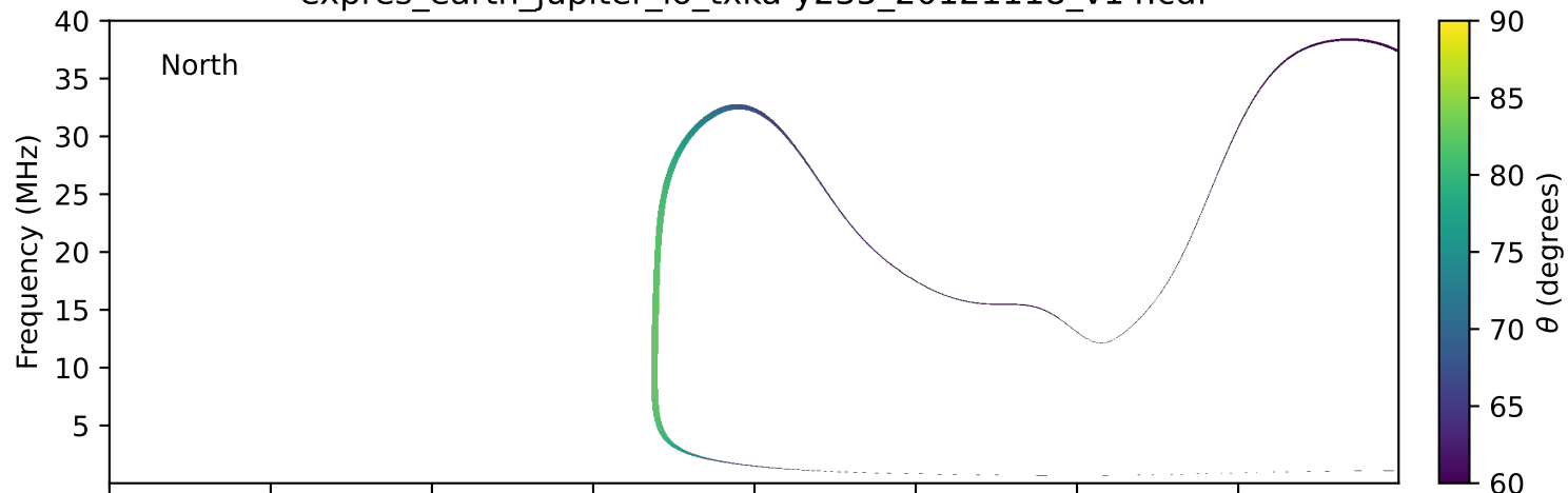
expres_earth_jupiter_io_txka-y235_20121118_v14.cdf
