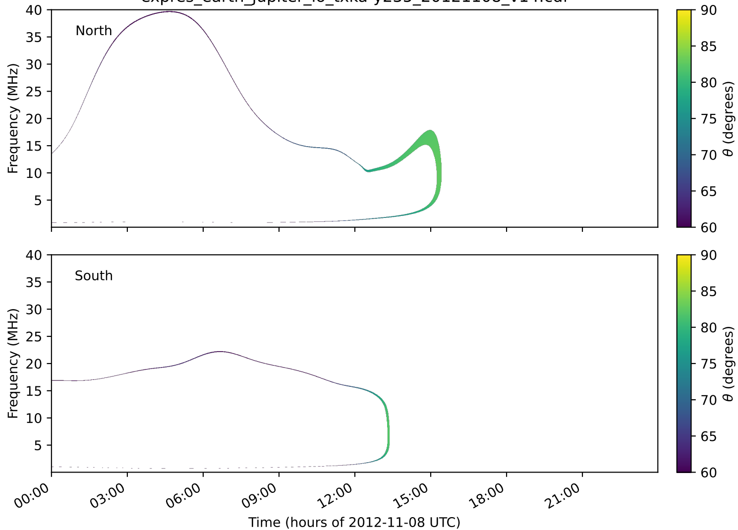
expres_earth_jupiter_io_txka-y235_20121108_v14.cdf
