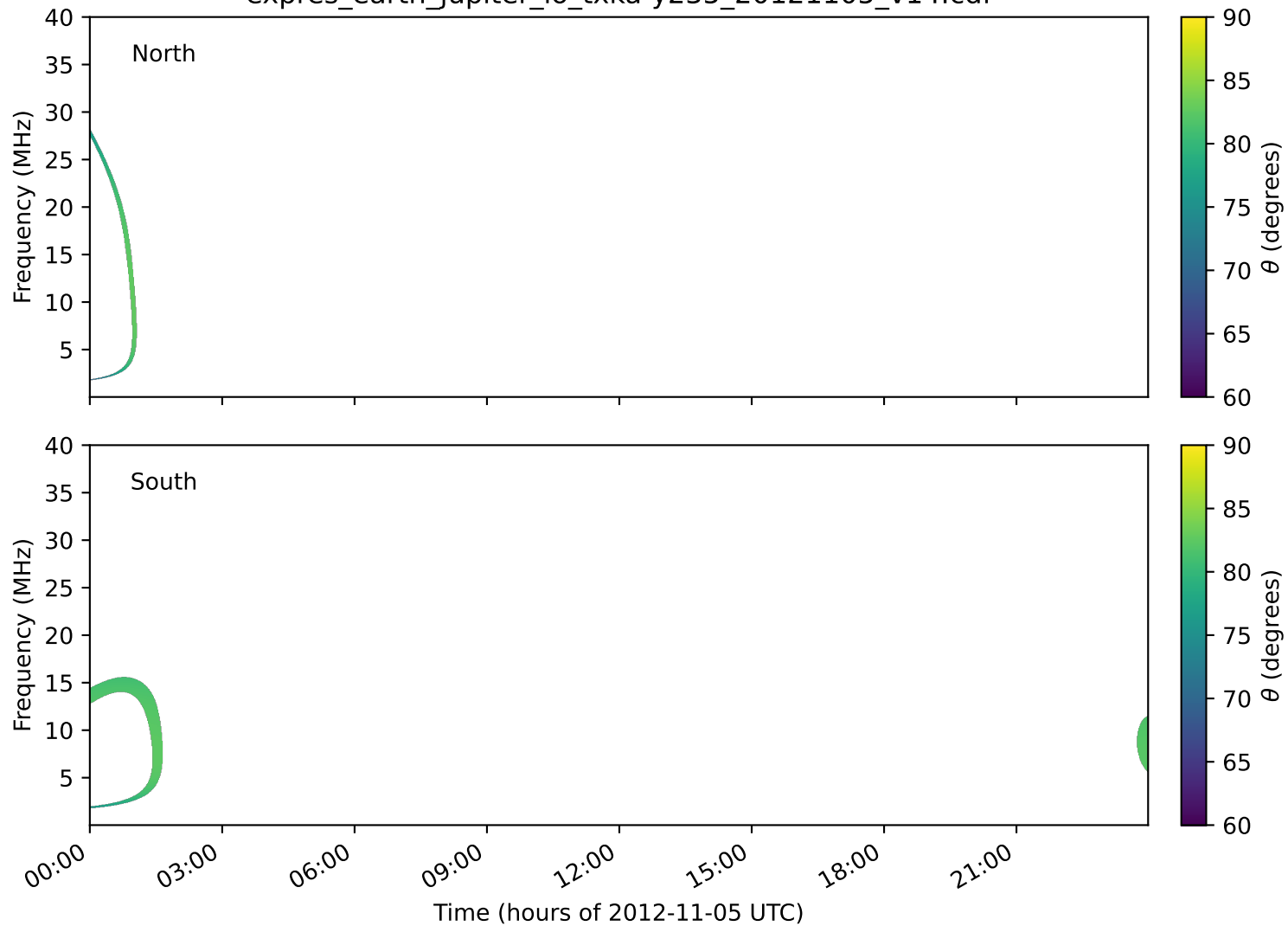
expres_earth_jupiter_io_txka-y235_20121105_v14.cdf
