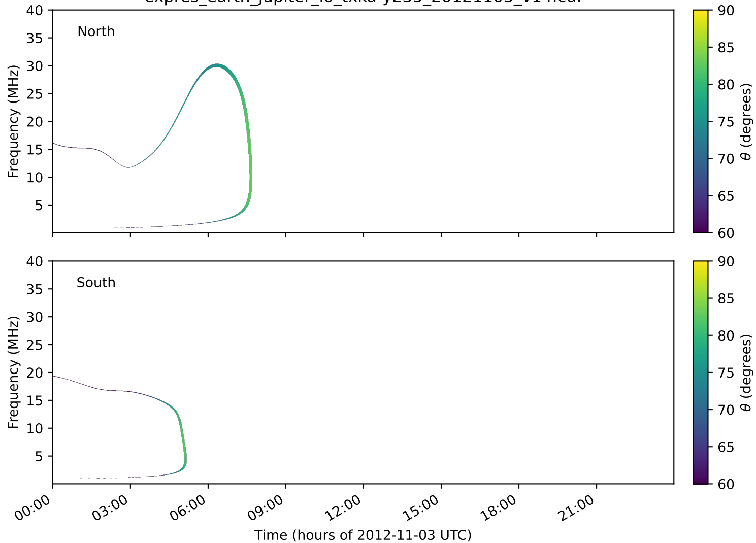
expres_earth_jupiter_io_txka-y235_20121103_v14.cdf
