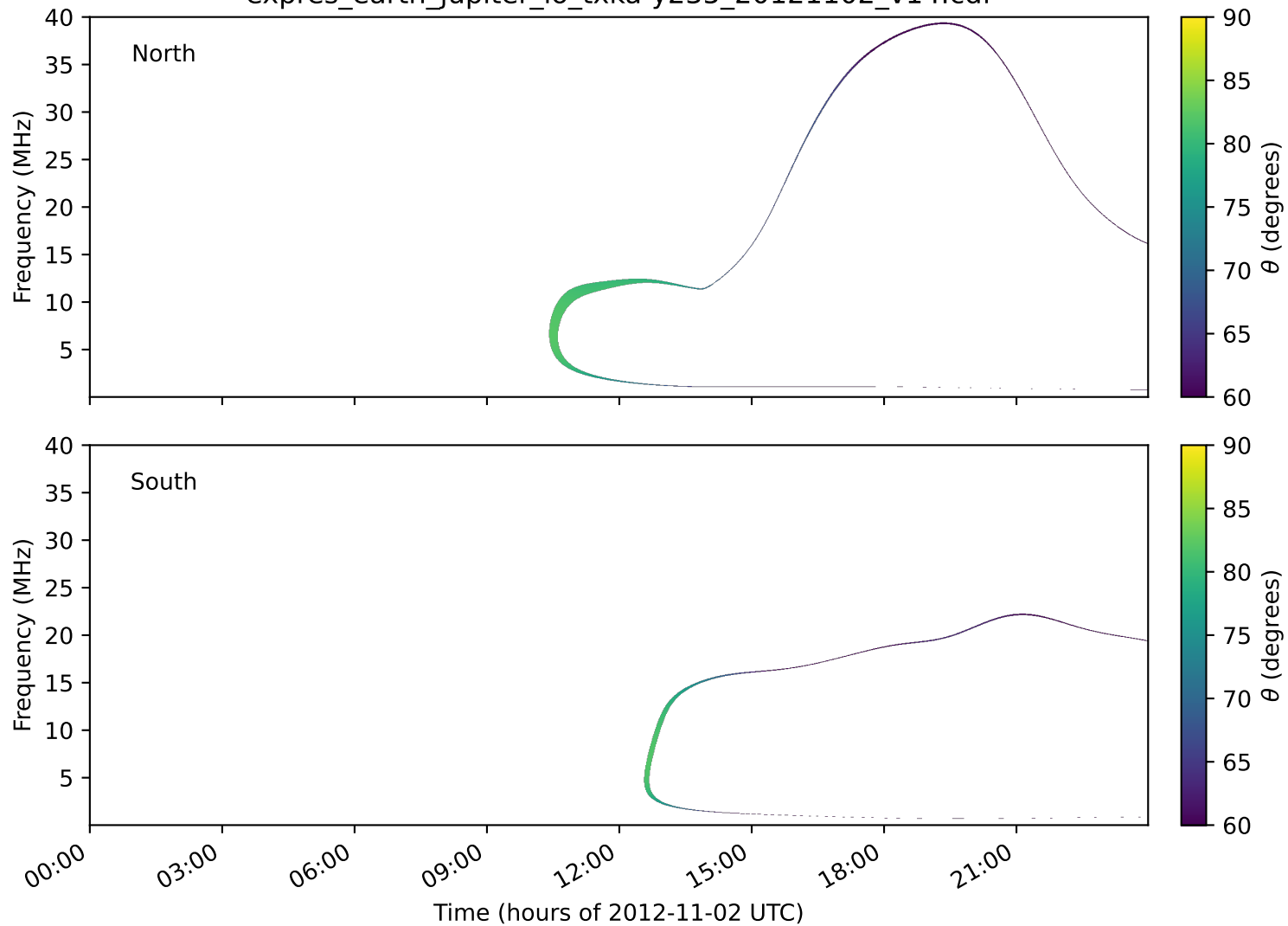
expres_earth_jupiter_io_txka-y235_20121102_v14.cdf
