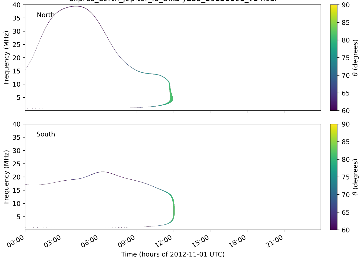
expres_earth_jupiter_io_txka-y235_20121101_v14.cdf
