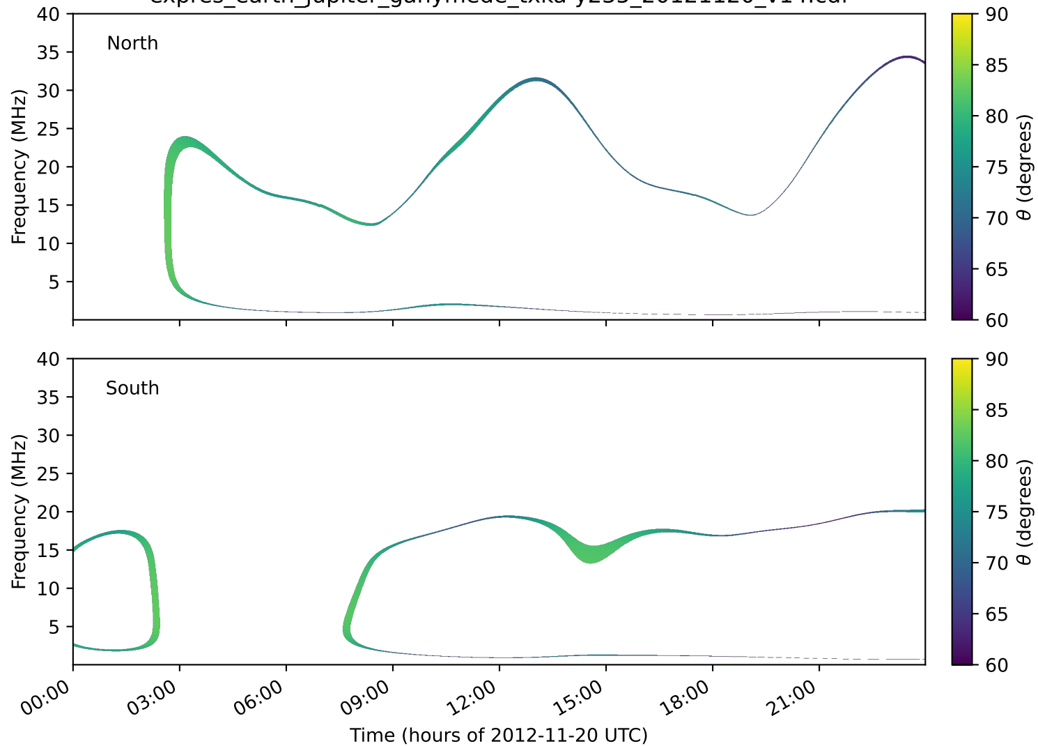
expres_earth_jupiter_ganymede_txka-y235_20121120_v14.cdf
