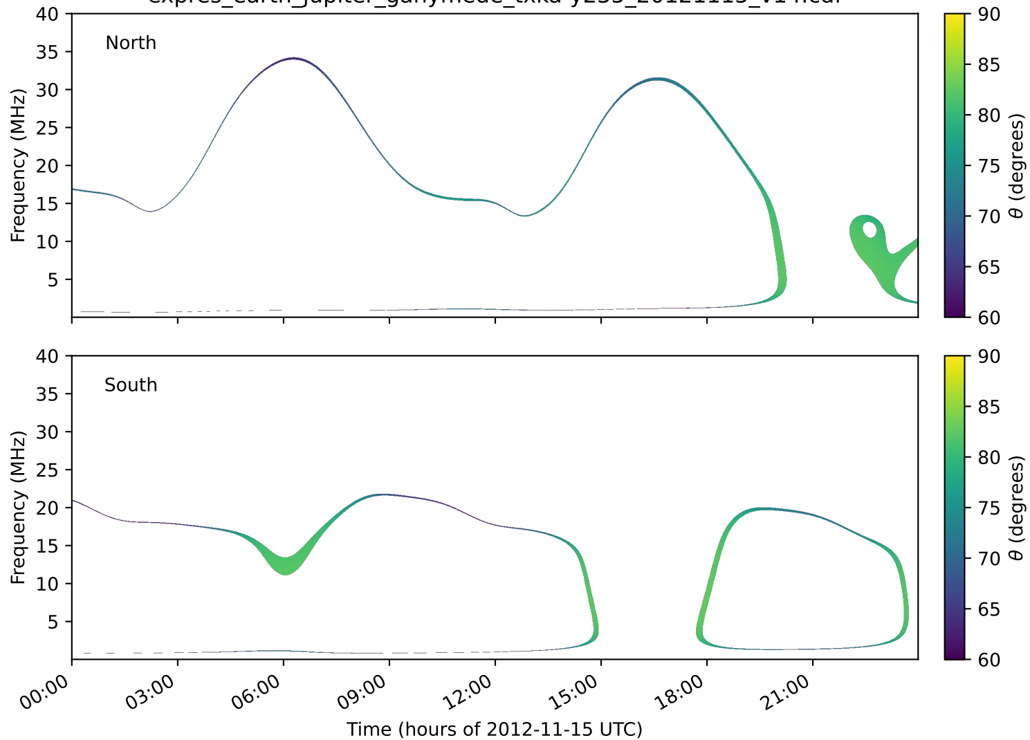
expres_earth_jupiter_ganymede_txka-y235_20121115_v14.cdf
