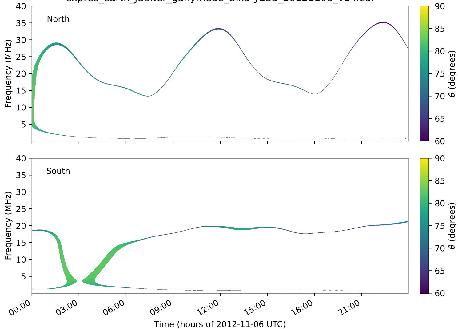
expres_earth_jupiter_ganymede_txka-y235_20121106_v14.cdf
