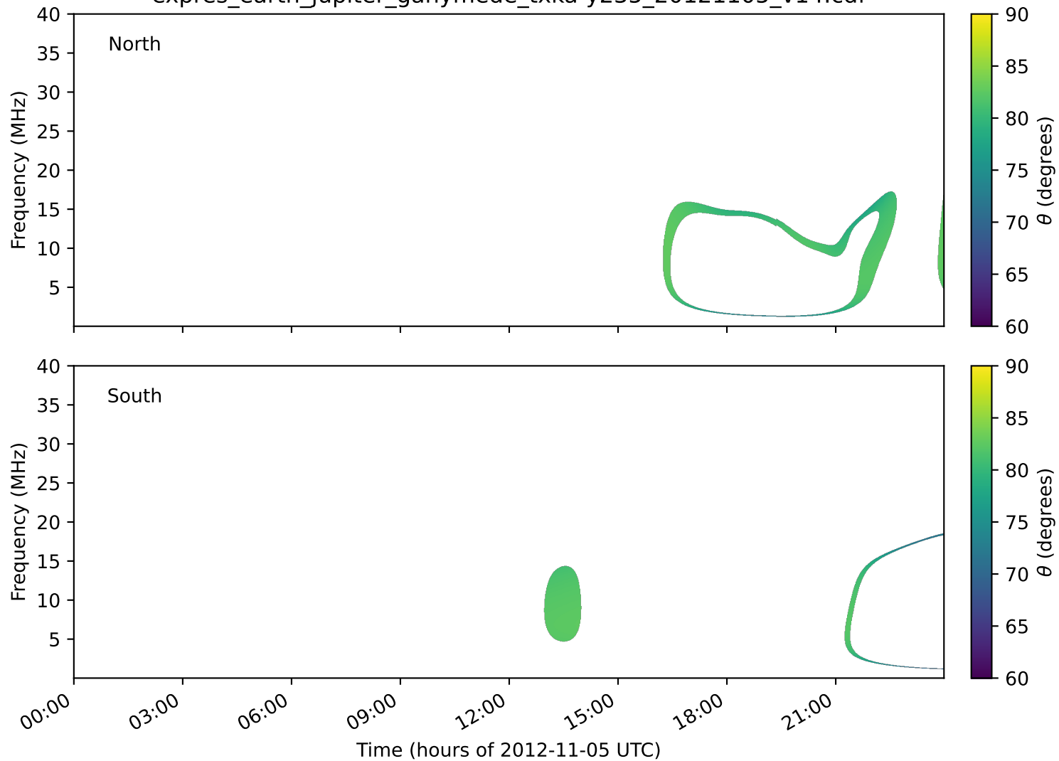
expres_earth_jupiter_ganymede_txka-y235_20121105_v14.cdf
