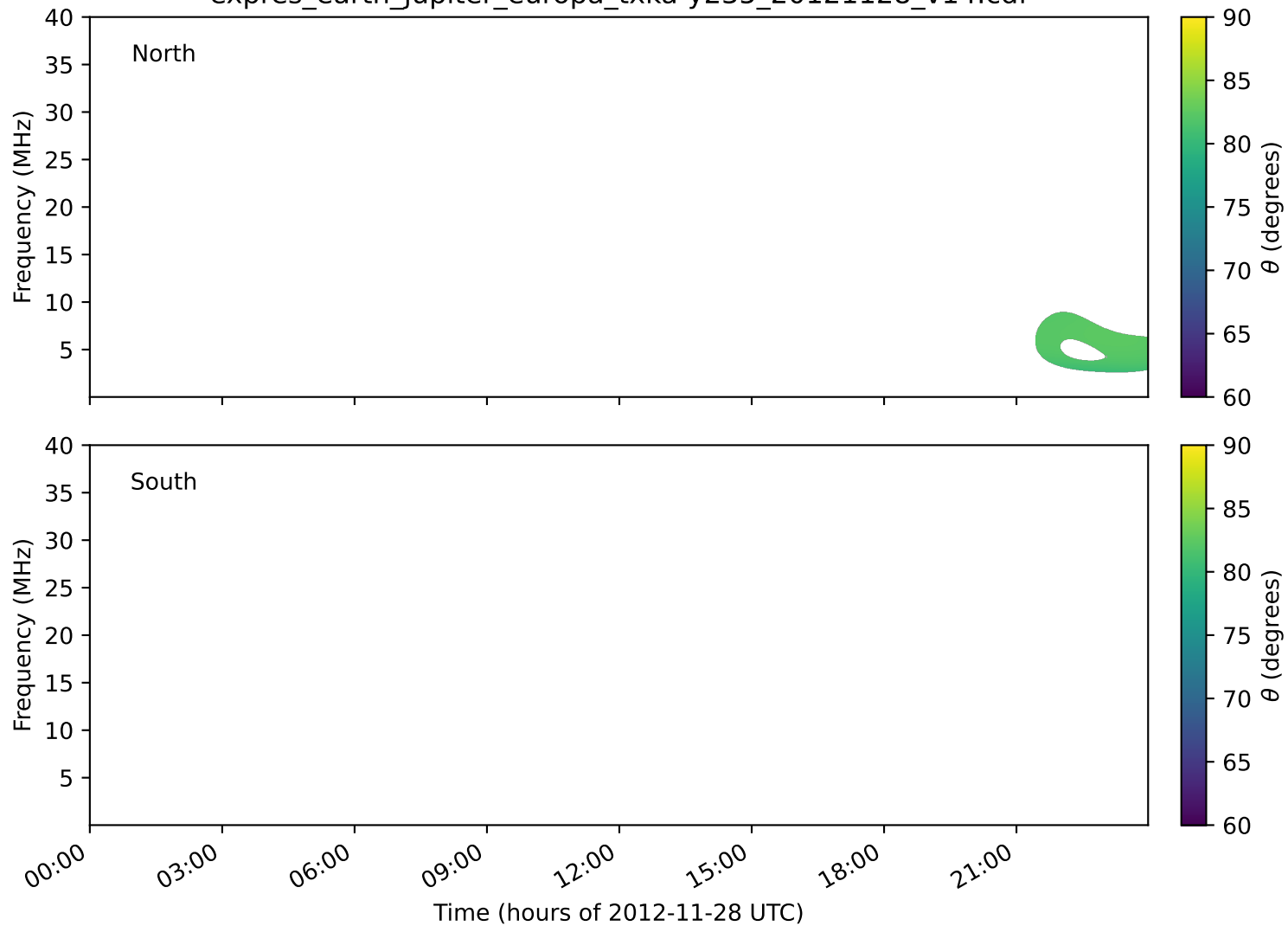
expres_earth_jupiter_europa_txka-y235_20121128_v14.cdf
