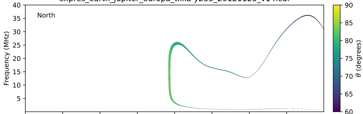
expres_earth_jupiter_europa_txka-y235_20121125_v14.cdf
