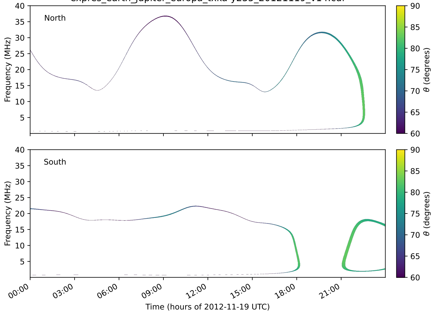
expres_earth_jupiter_europa_txka-y235_20121119_v14.cdf
