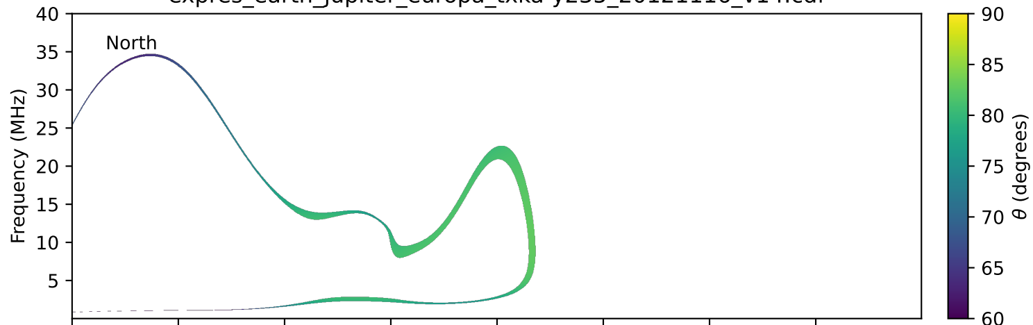
expres_earth_jupiter_europa_txka-y235_20121116_v14.cdf
