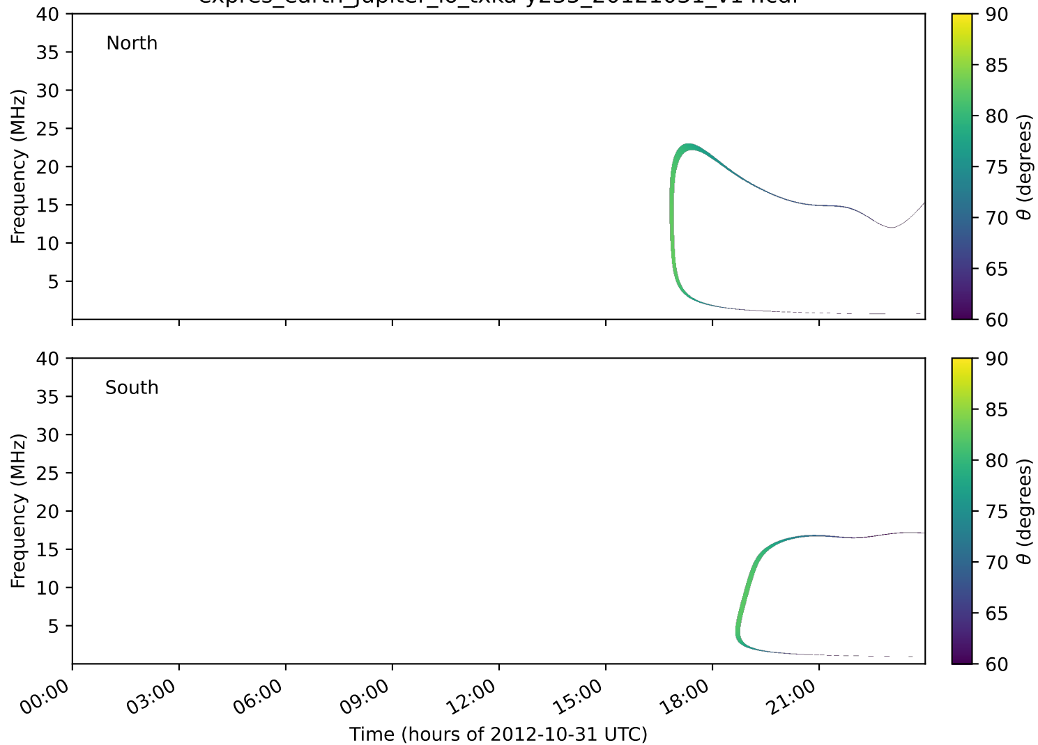
expres_earth_jupiter_io_txka-y235_20121031_v14.cdf
