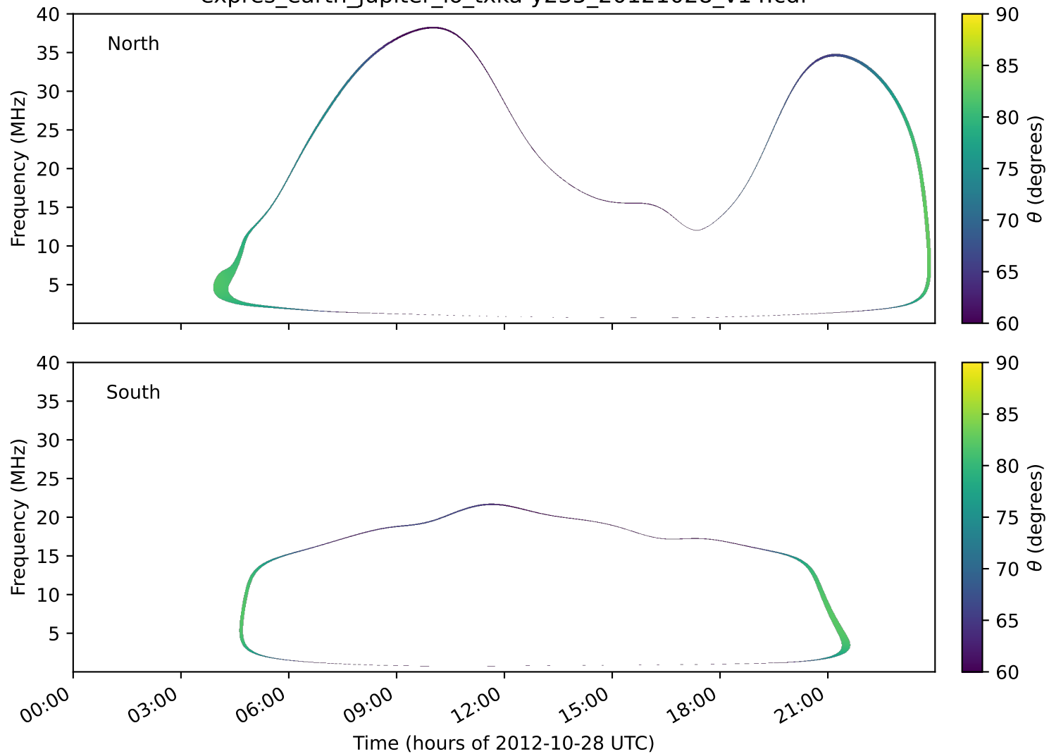
expres_earth_jupiter_io_txka-y235_20121028_v14.cdf
