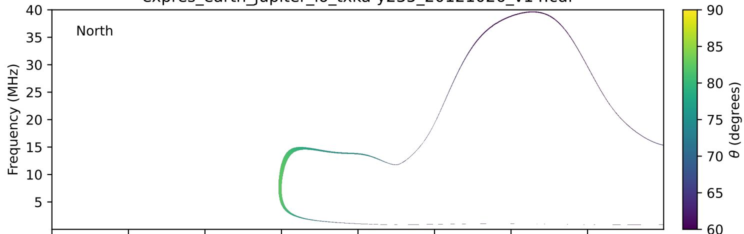
expres_earth_jupiter_io_txka-y235_20121026_v14.cdf
