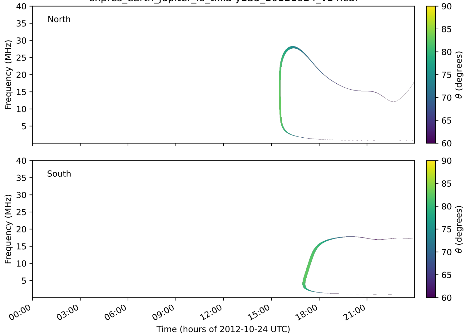
expres_earth_jupiter_io_txka-y235_20121024_v14.cdf
