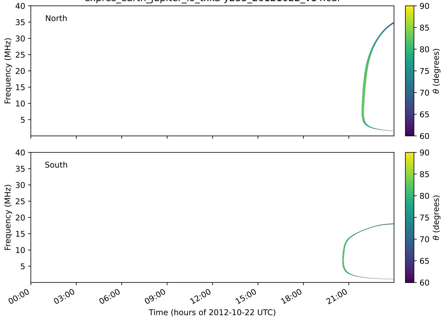
expres_earth_jupiter_io_txka-y235_20121022_v14.cdf
