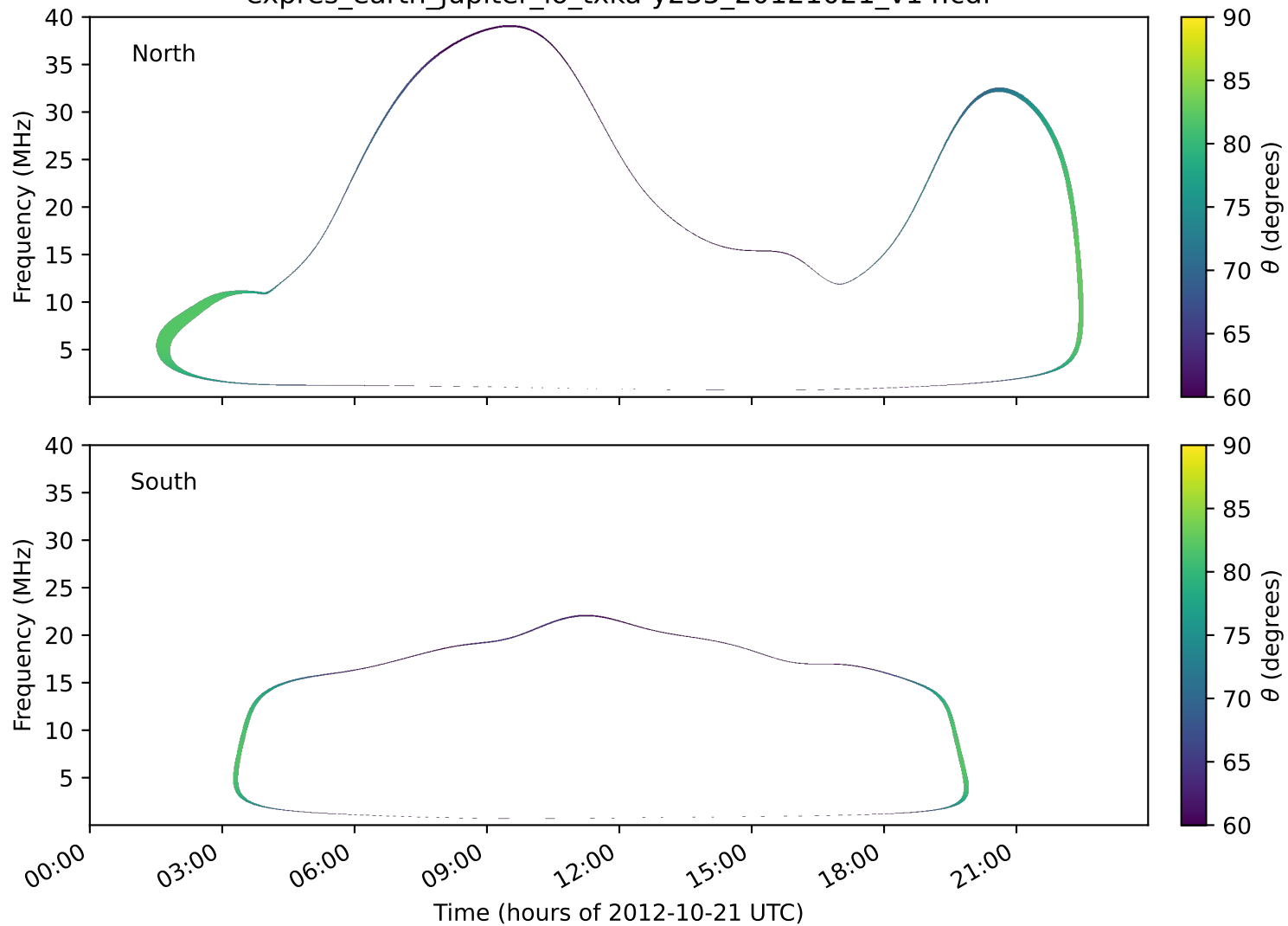
expres_earth_jupiter_io_txka-y235_20121021_v14.cdf
