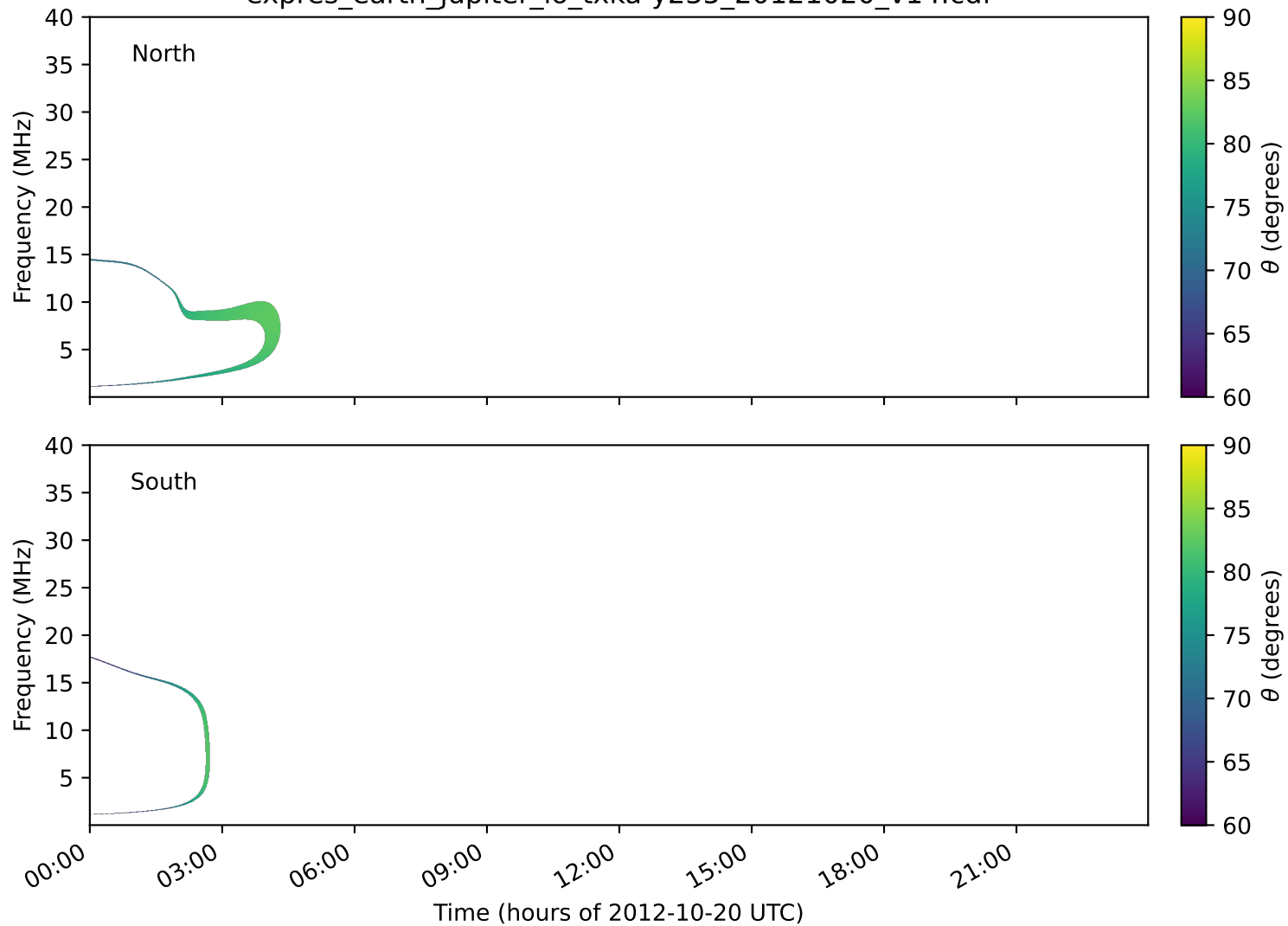
expres_earth_jupiter_io_txka-y235_20121020_v14.cdf
